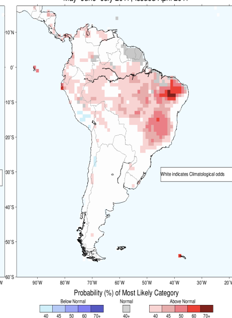
IRI Multi-Model Probability Forecast for Temperature for May-June-July 2017, Issued April 2017
