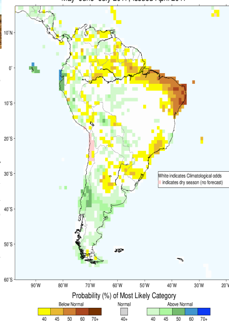
IRI Multi-Model Probability Forecast for Precipitation for May-June-July 2017, Issued April 2017
