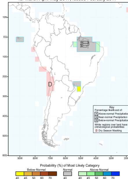
IRI Multi-Model Probability Forecast for Precipitation for March-April-May 2017, Issued February 2017
