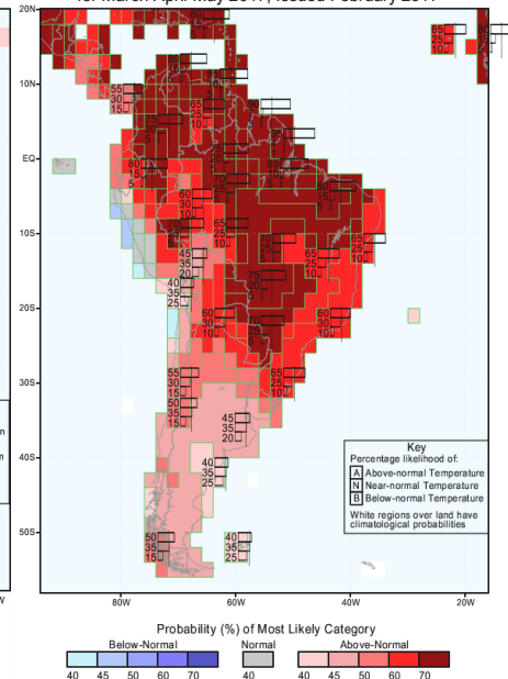
IRI Multi-Model Probability Forecast for Temperature for March-April-May 2017, Issued February 2017
