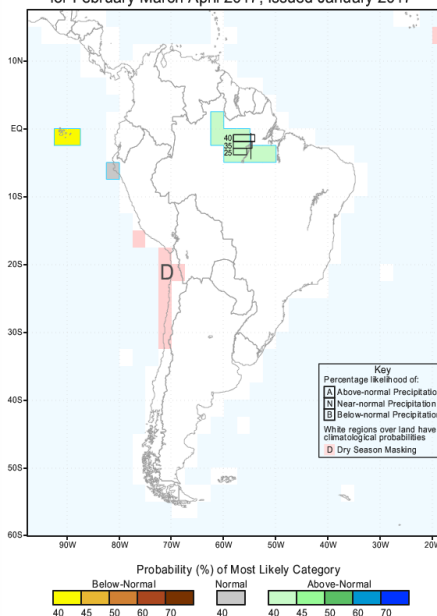
IRI Multi-Model Probability Forecast for Precipitation for February-March-April 2017, Issued January 2017
