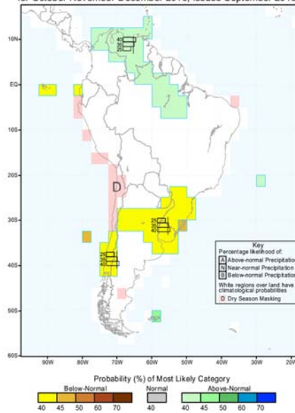
IRI Multi-Model Probability Forecast for Precipitation for October-November-December 2016, Issued September 2016
