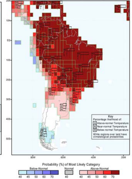
IRI Multi-Model Probability Forecast for Temperature for October-November-December 2016, Issued September 2016
